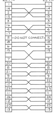
CABLE WIRING DIAGRAM
