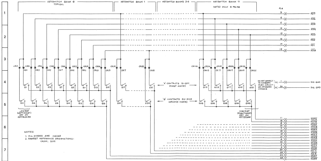
FENDER MI CHROMA POLARIS KEYBOARD SCHEMATIC
